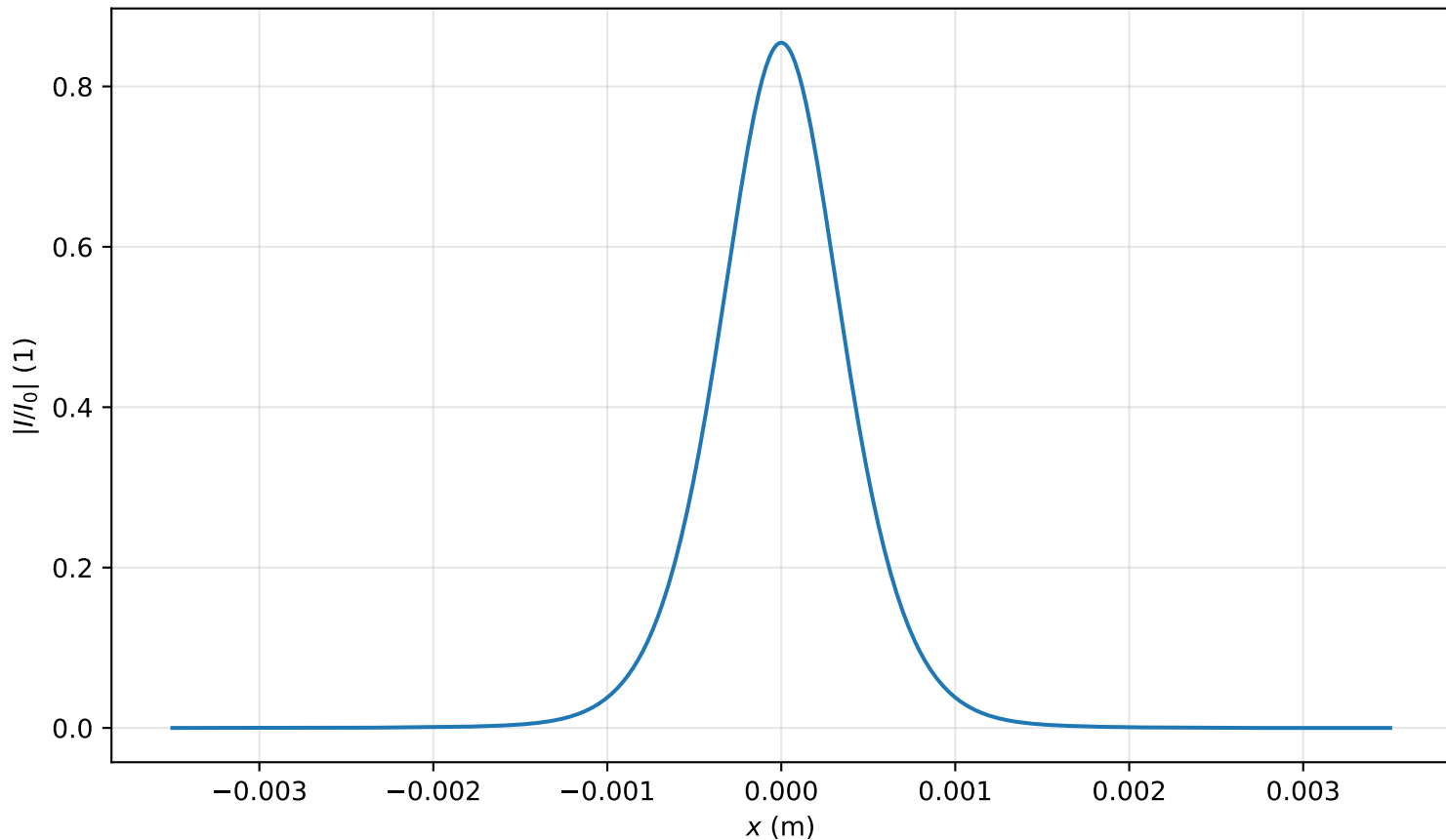
Intensity profile I(x, y = 0, z = 2.946m)/I_0 , P_{in}=0.7P_{cr} , artificial time
